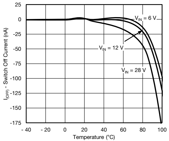
Fig. 11 - Switch OFF Current vs. Temperature
