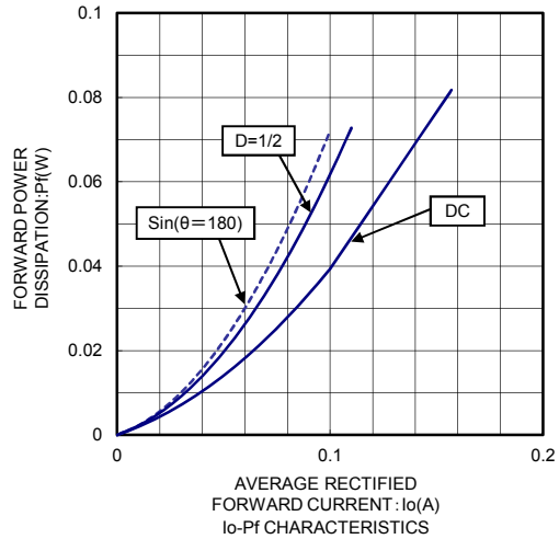
I o -Pf CHARACTERISTICS
