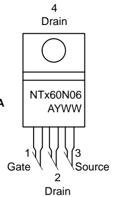
TO-220 CASE 221A STYLE 5
