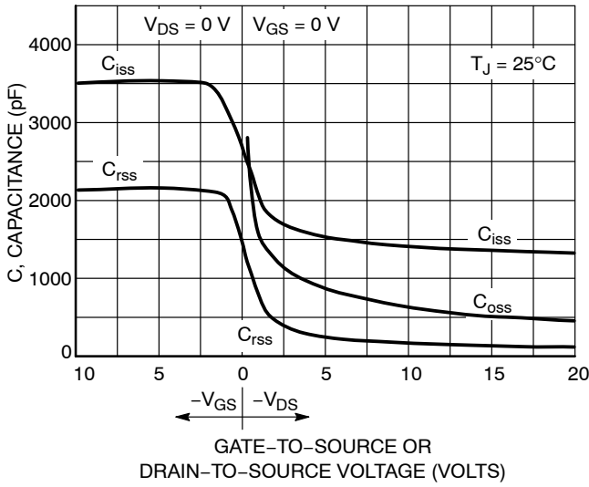
Figure 7. Capacitance Variation
