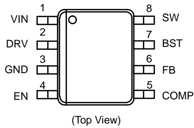
Figure 3. Pin Connections
