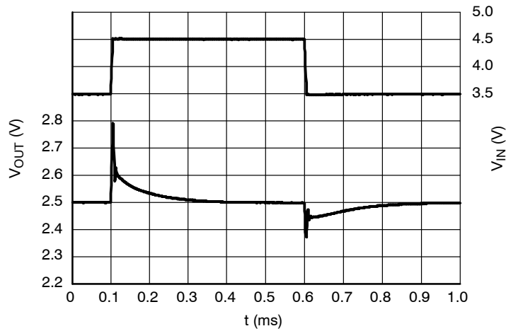
Figure 24. Line Transients, 2.5 V Version, t_R = t_F = 5 \mu\text{s} , I_{\text{OUT}} = 30 \text{ mA}
