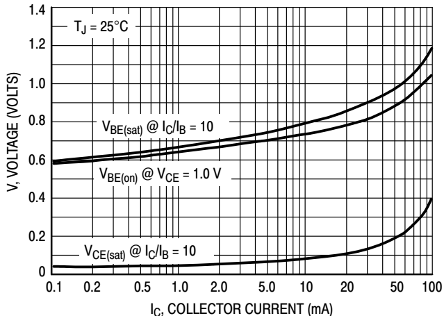
Figure 10. "On" Voltages
