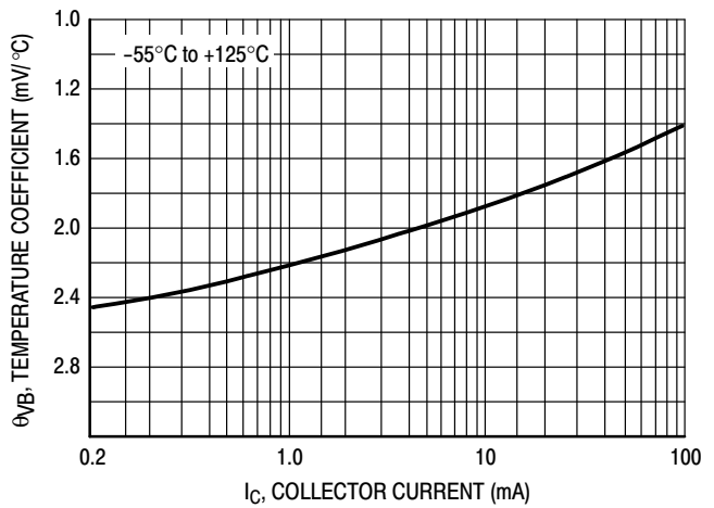
Figure 38. Base-Emitter Temperature Coefficient
