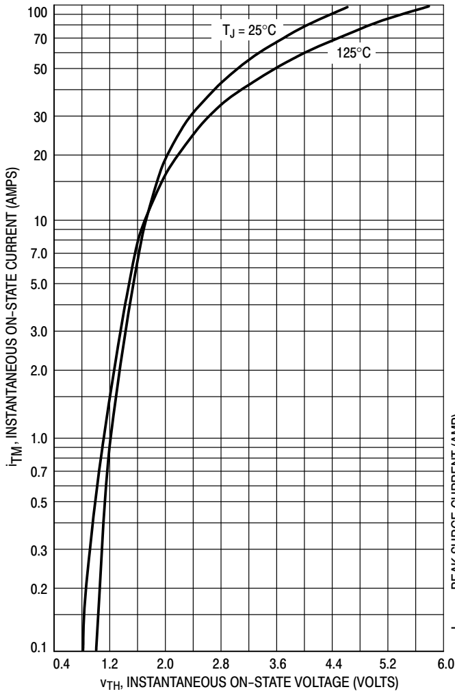
Figure 3. On-State Characteristics
