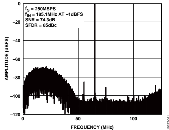
Figure 45. 22% Bandwidth Mode, Tuning Word = 41
