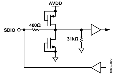
Figure 20. Equivalent SDIO Circuit
