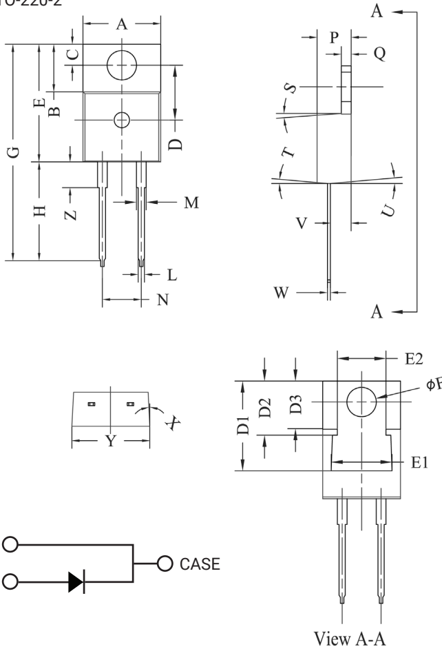
Package TO-220-2
