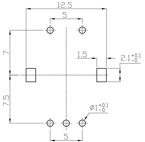
P.C.B.MOUNTING DETAIL
