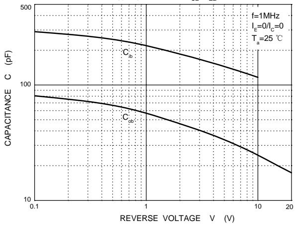
C_{ob}/C_{ib} — V_{CB}/V_{EB}
